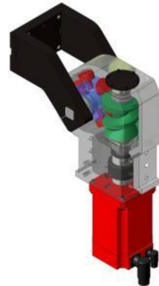
New Servo Electric Power Pivot
