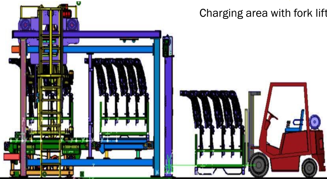
Container changing system in which the full container are led to the robot and the empty containers are transported to the removal.
