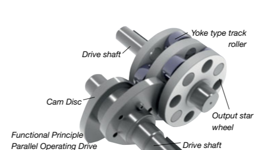
Functional Principle Parallel Operating Drive
